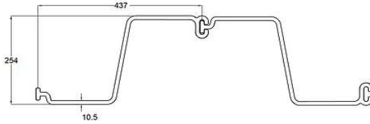
ESC VINYL SHEET PILE PROFILE ESC-VZ437-10.5
