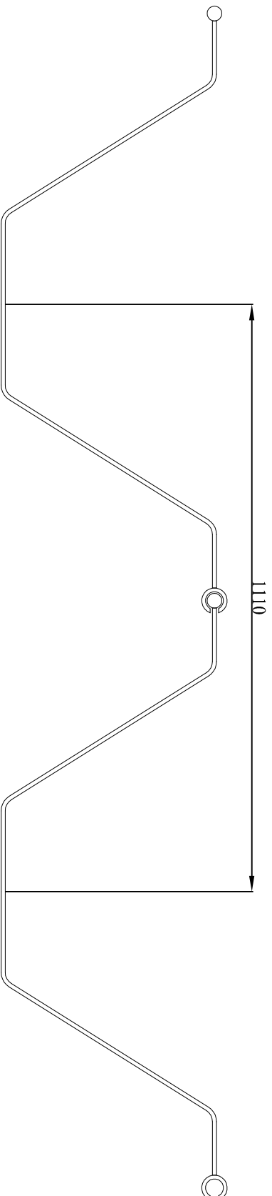
INTERLOCKED PROFILE
