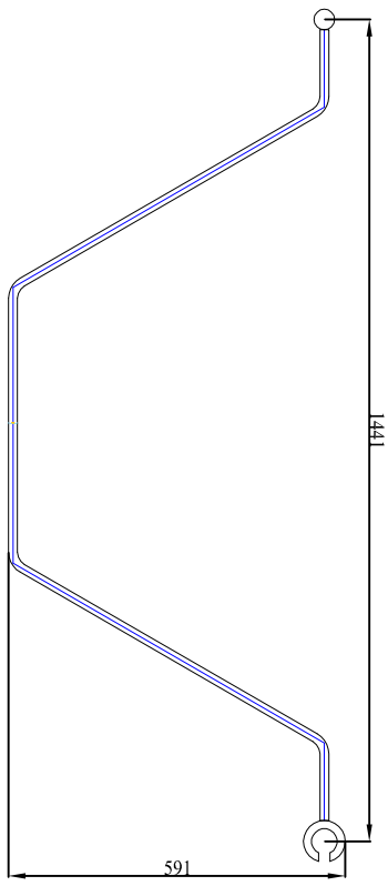
SHEET PILE PROFILE
