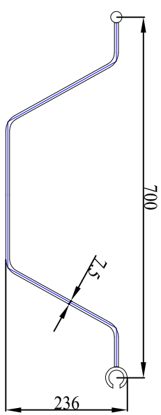
SHEET PILE PROFILE
